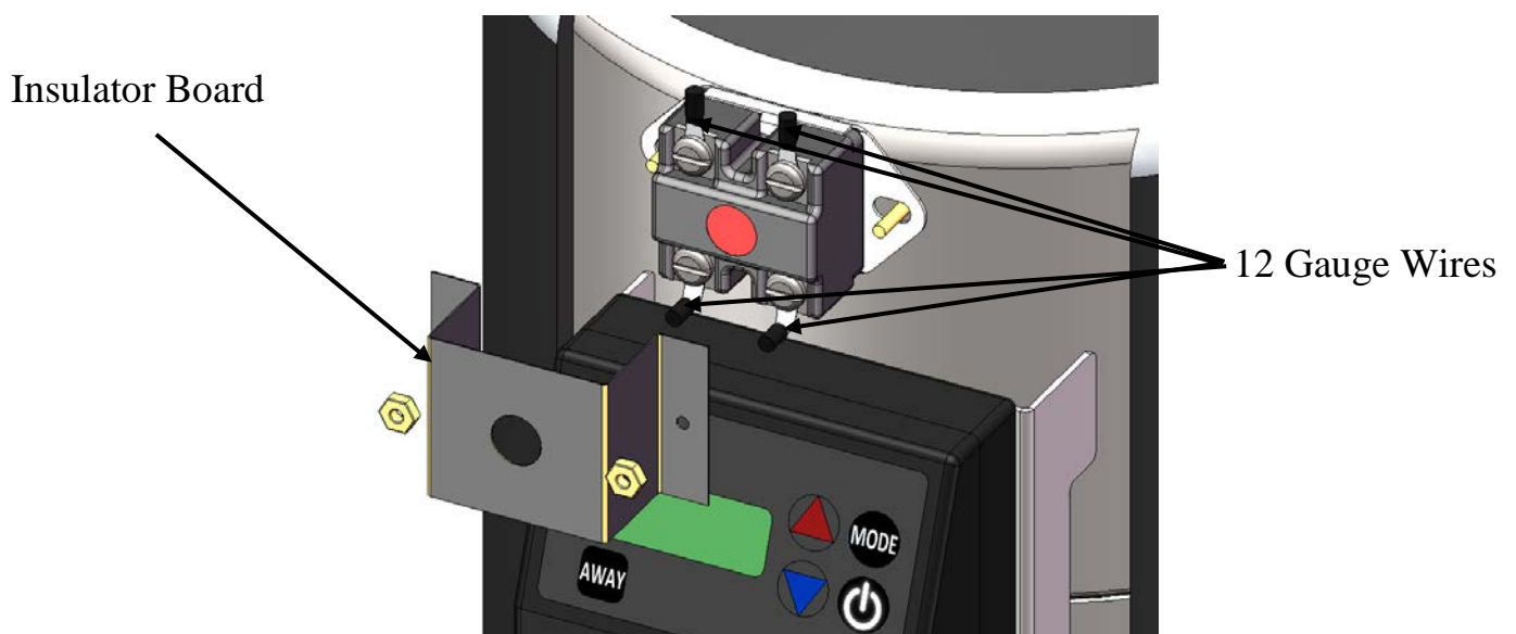
Figure 10: Hi-Limit Replacement
