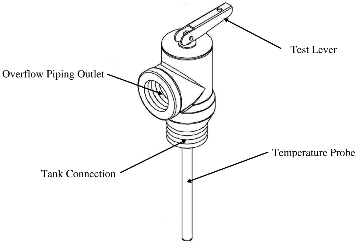
Figure 13: Relief Valve
