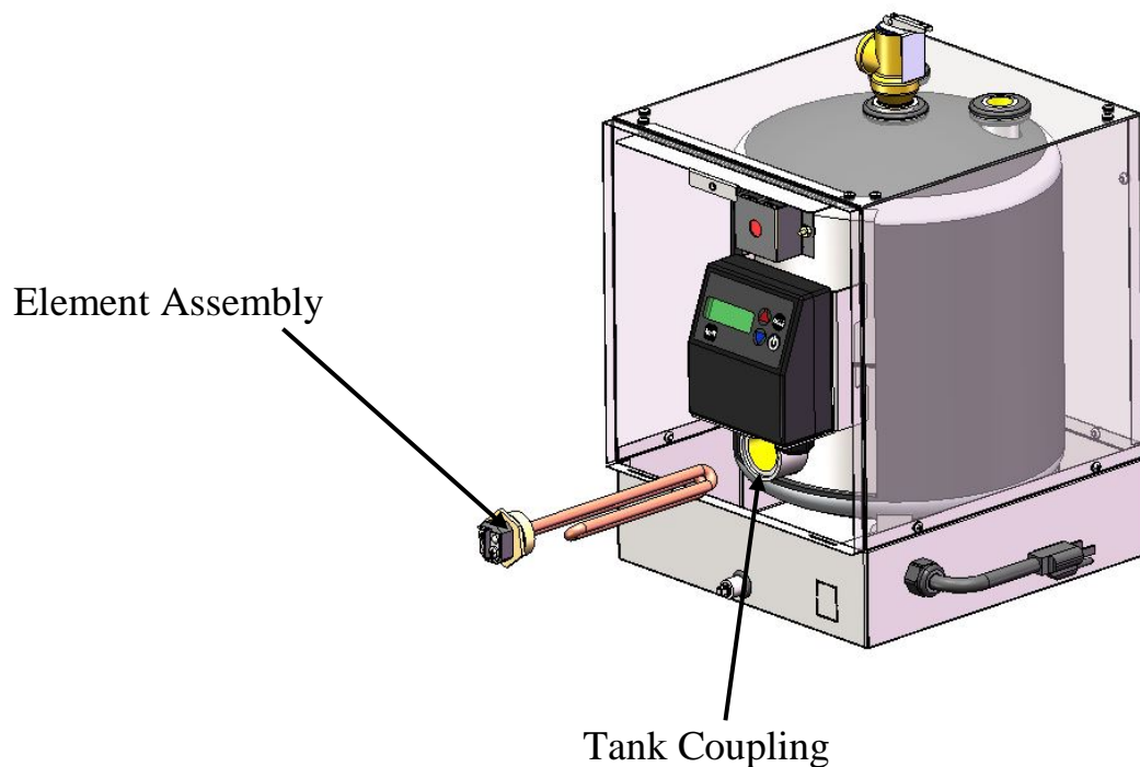
Figure 12: Remove Heating Element
