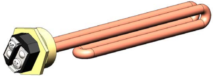
Figure 2: Heating Element
