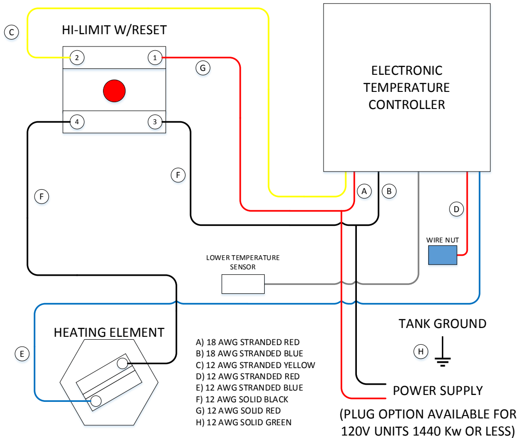
Figure 7 - Wiring Diagram
