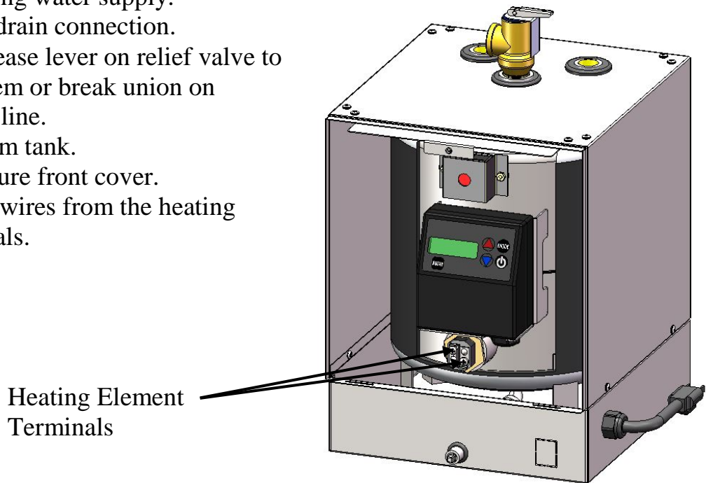
Figure 11: Heating Element Terminals
