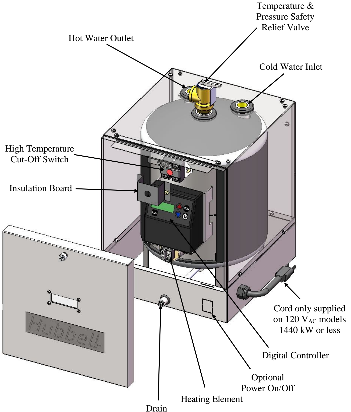
Figure 1: Part Locations
