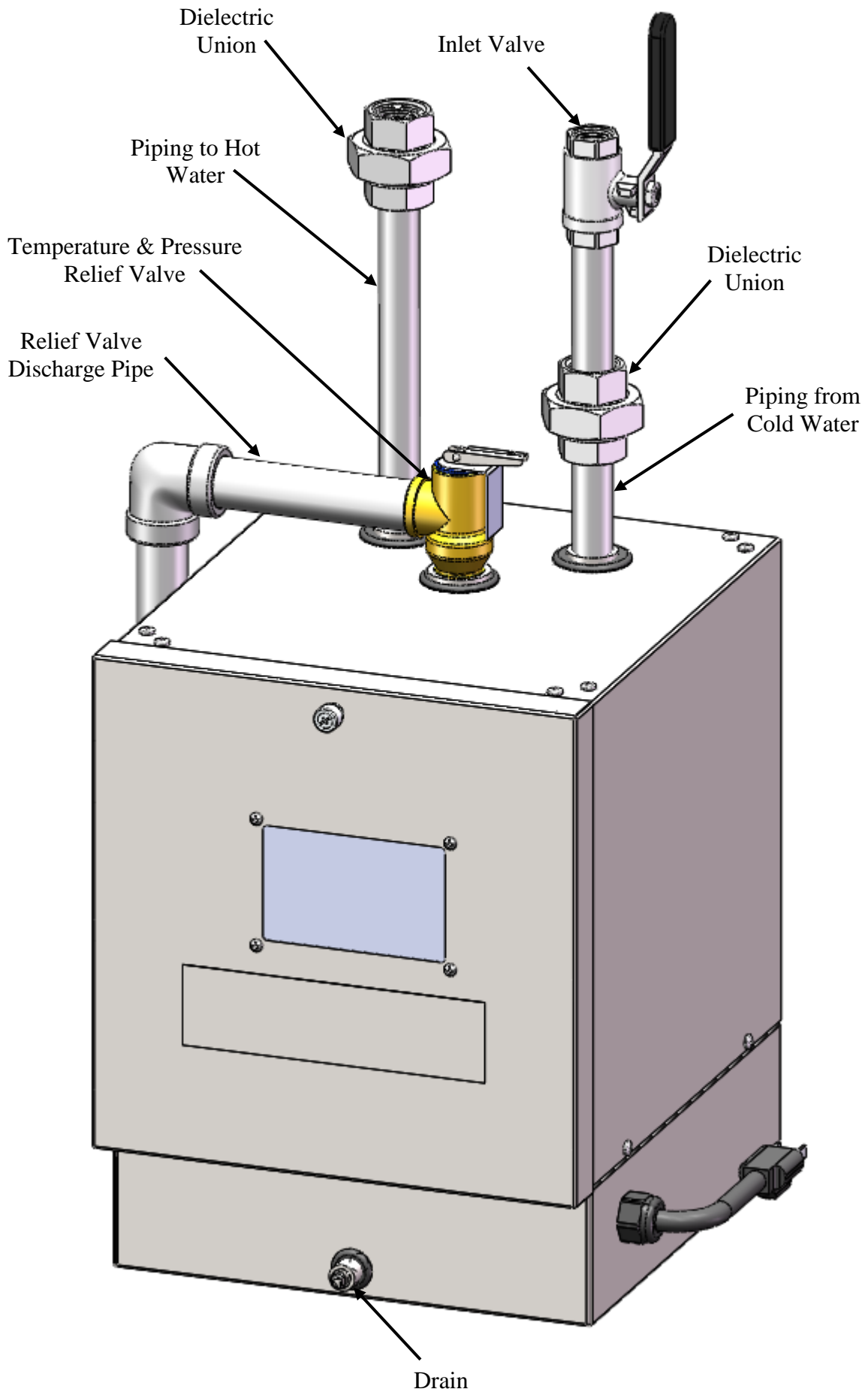
Figure 8: Recommended Installation Diagram
